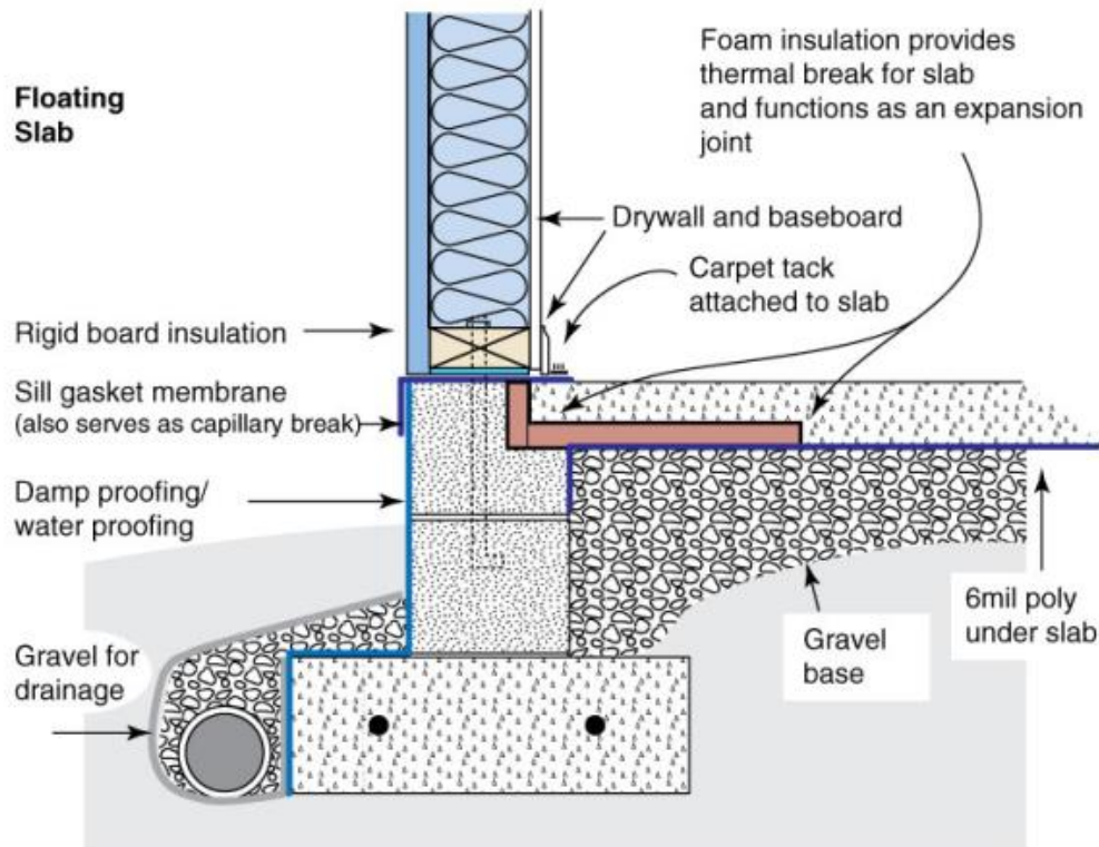
Figure 60: Slab edge insulation for floating slab
