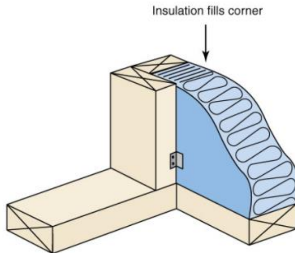
Figure 61: Insulated corner
